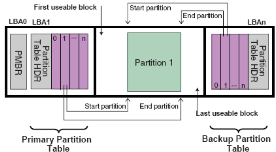
Figure 11-2. GUID Partition Table (GPT) Scheme
